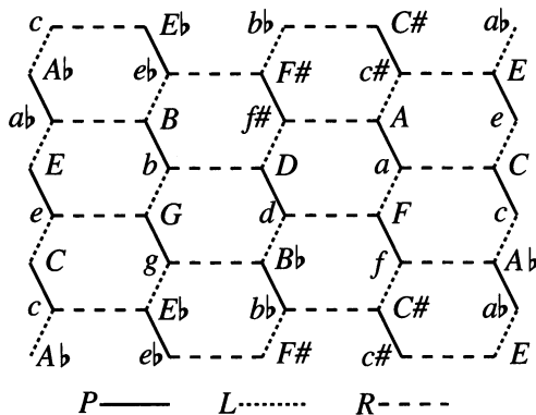
Figure 6. Douthett and Steinbach’s graph from [8].
