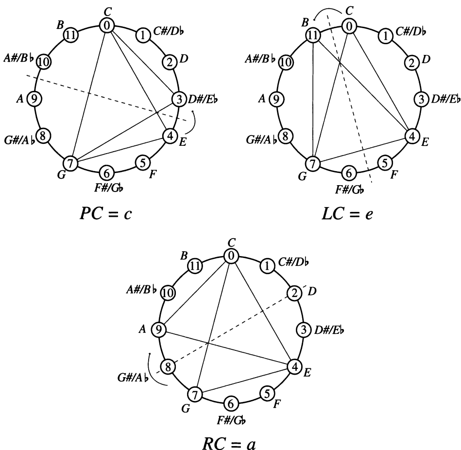
Figure 4. Minimal motion of the moving voice under P , L , and R .
