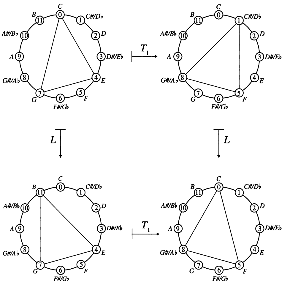
Figure 8. Illustration of commutativity of T_1 and L .
