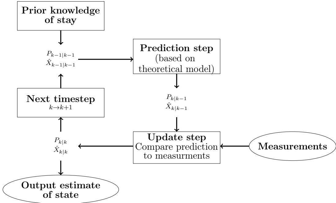
RYSUNEK 2. Principle of a Kalman filter
